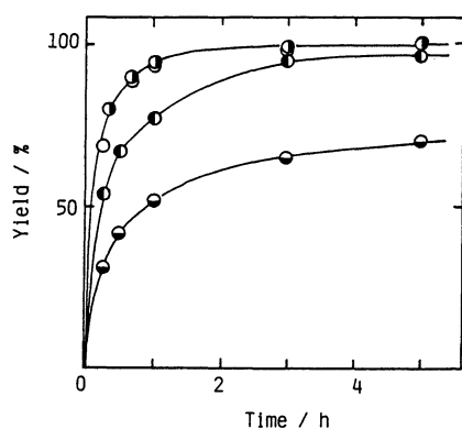
Fig. 5. Effect of ion content on the activity of silica gel-supported 3-4, Br toward decyl mesylate. ○, 0.25; ◐, 0.50; ●, 1.00; ●, 2.00 mmol g -1 .
